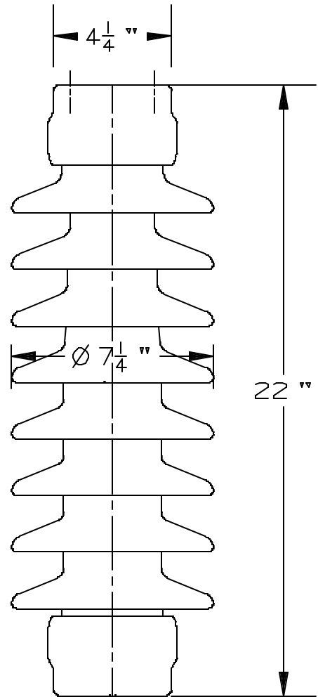
4 HOLES EACH END 1/2-13 +.015" ON Ø3" B.C.
